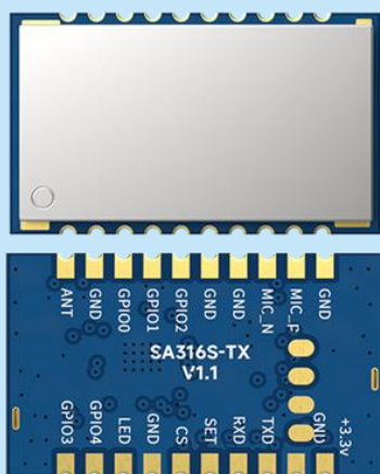
SA316S-TX
