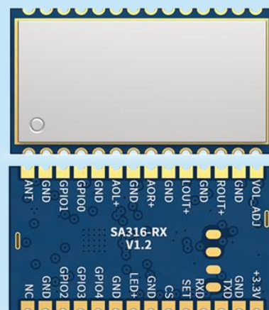
SA316-RX
